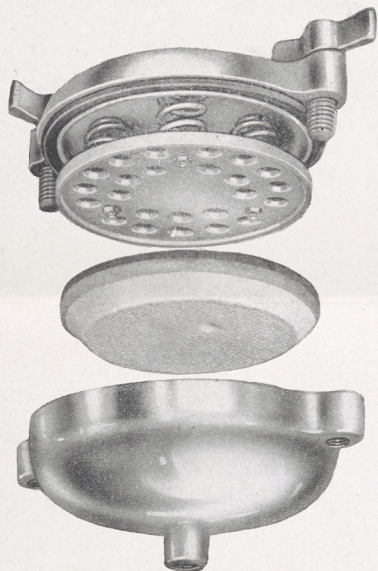
The SPA, open, showing simple construction and assembly
